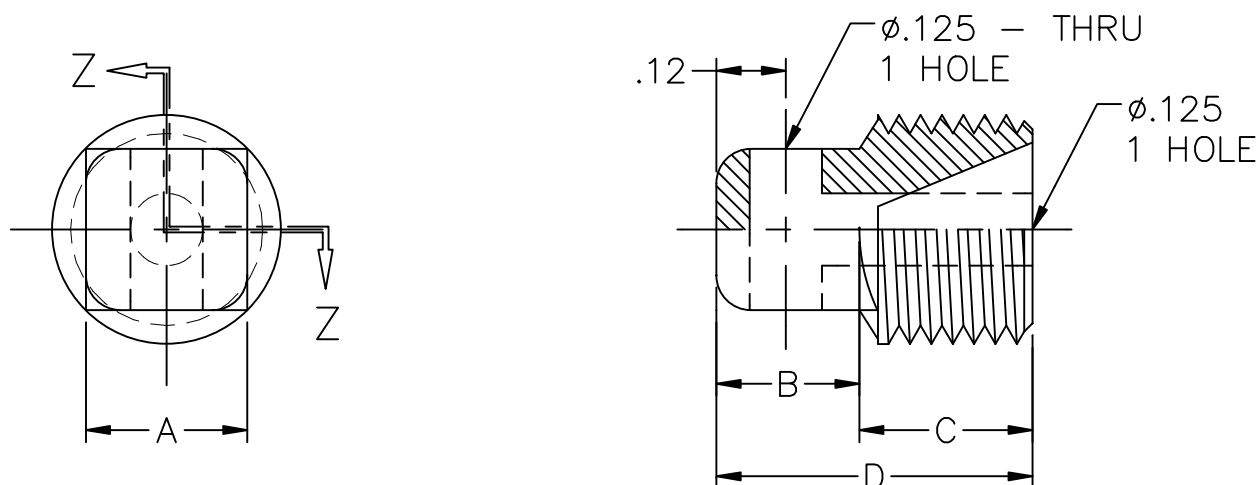
SECTION Z-Z
