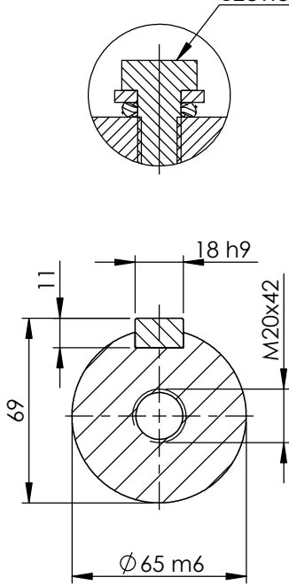
SECTION A-A SCALE 1 : 2.5
