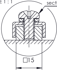
DETAIL B SCALE 1 : 1
