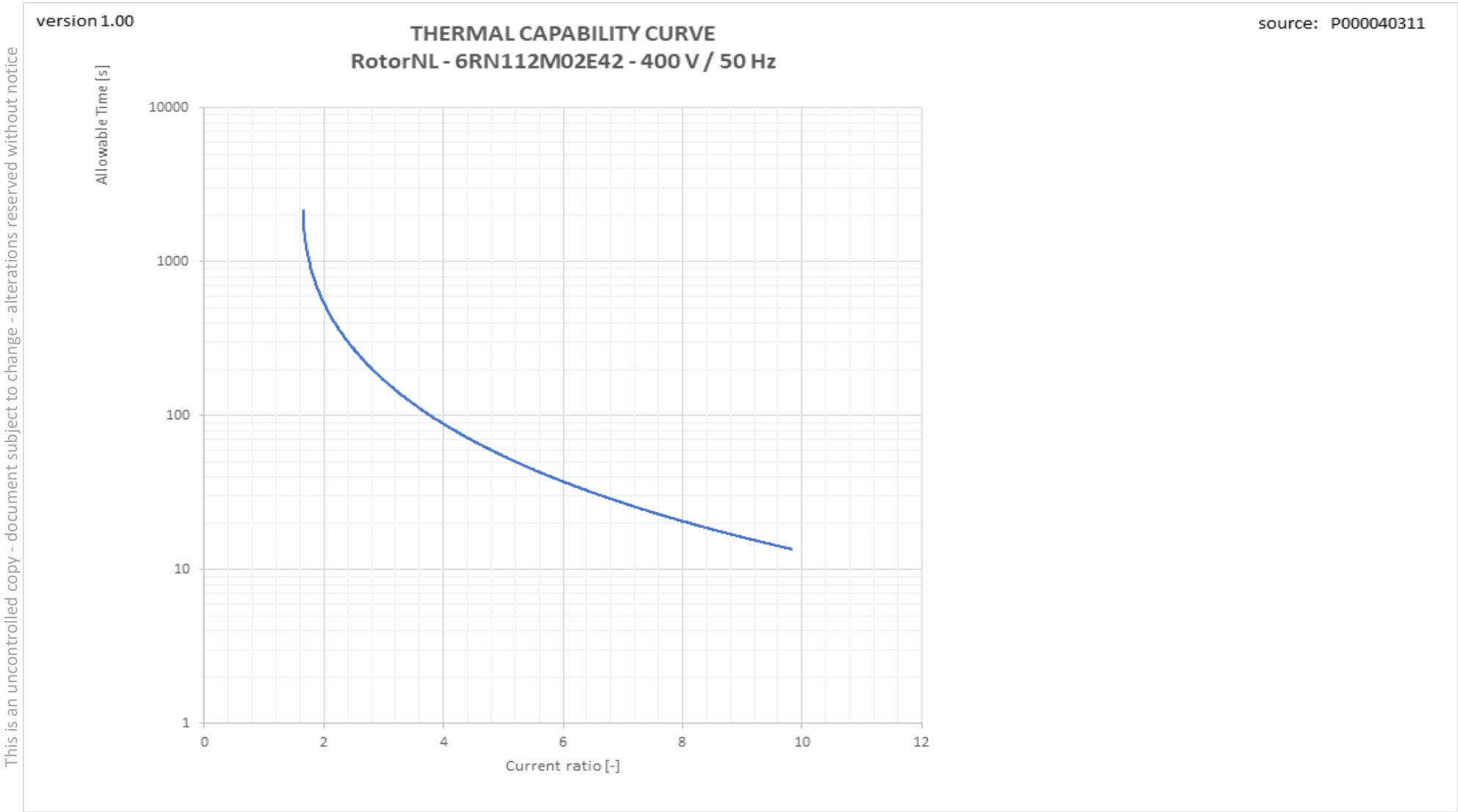
Therm_VSD graph
