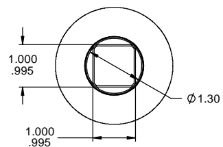
DETAIL A (SHAFT) SCALE 2:1
