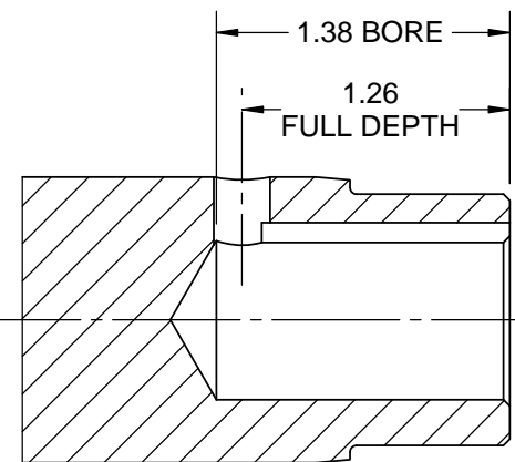
SECTION A-A SHAFT DETAIL
