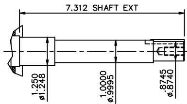
SHAFT DETAIL
