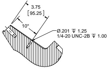
SECTION L-L 2PL (90° APART)
