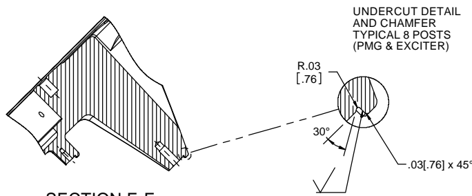
SECTION E-E
