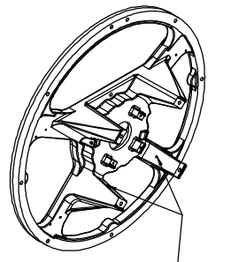
(2X 1/4-20 TAPPED HOLES - REFER TO SECTION L-L)
